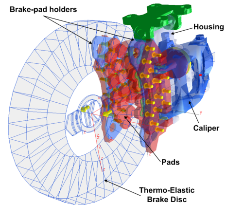
Figure 10: Braking mechanism of a train.
