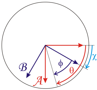
Figure 2: Coordinate transformation with angle \chi , that leads from the Lagrangian to the Eulerian description.
